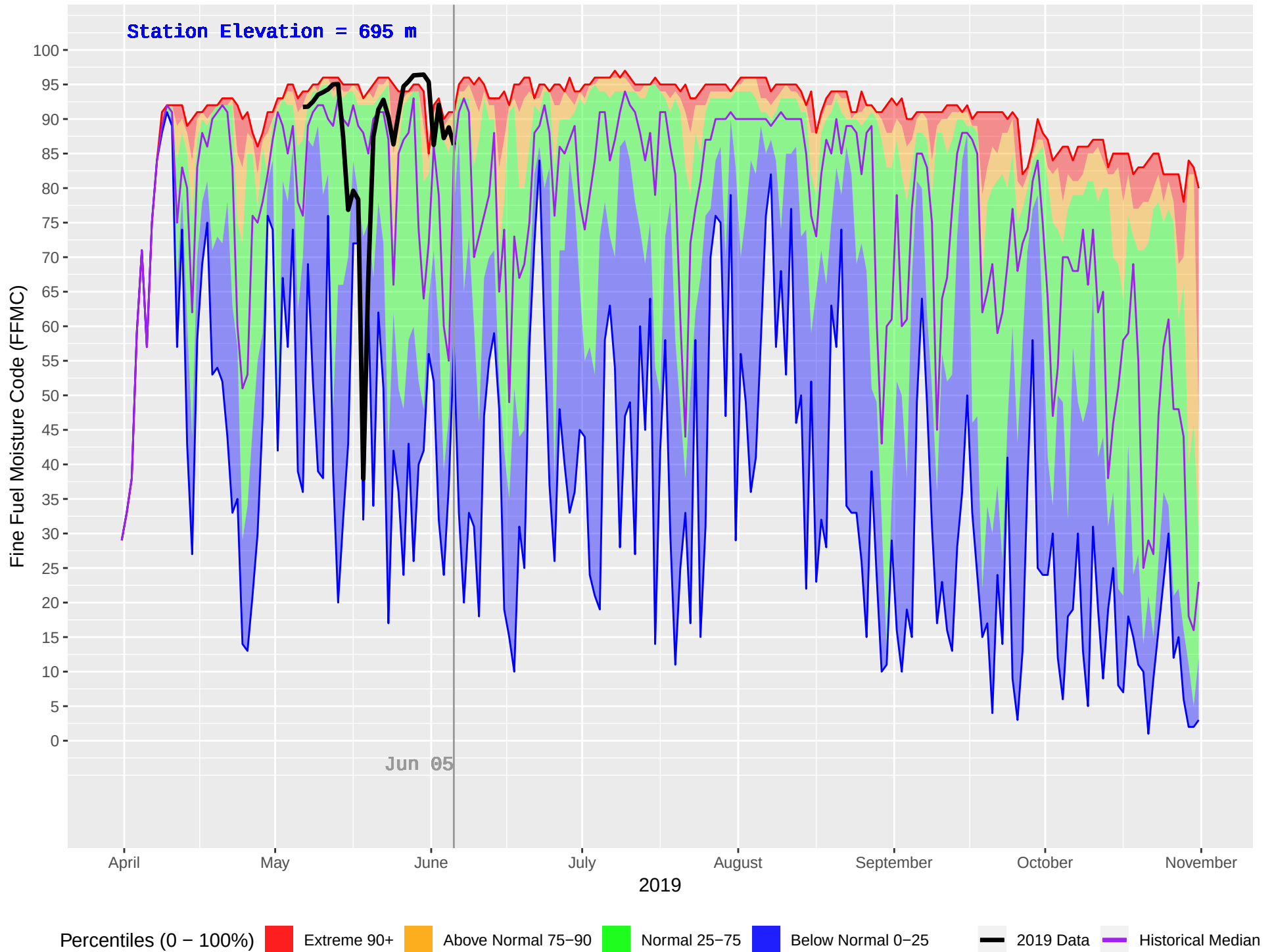
BLUE RIVER 2 (1108) : Historical (2011–2018) and Current (2019) Daily Fine Fuel Moisture Code (FFMC)
