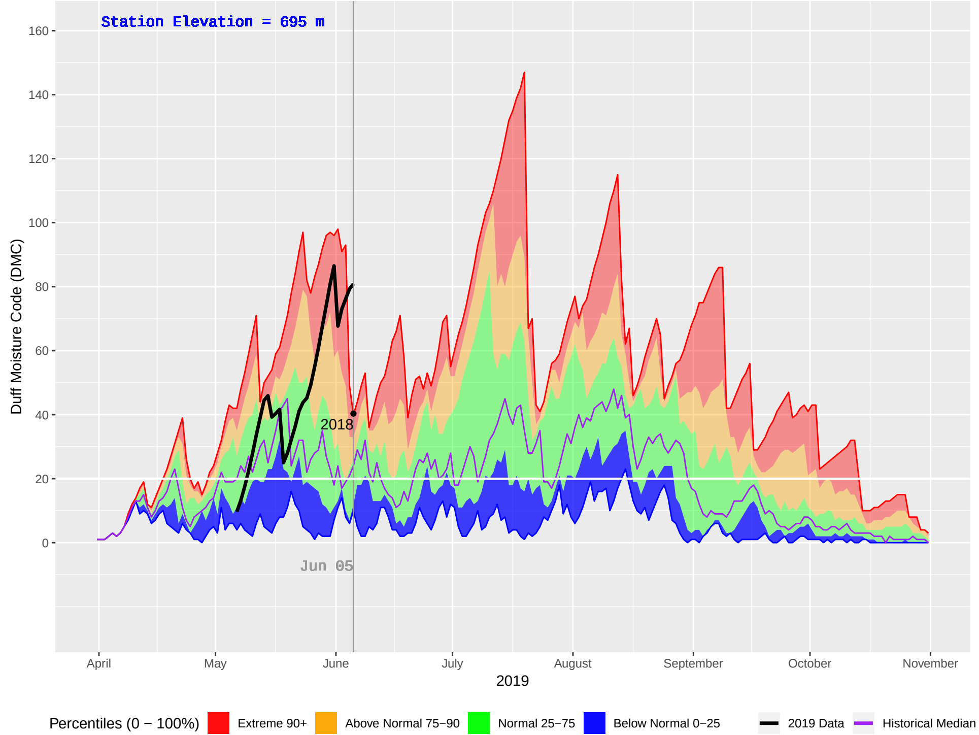
BLUE RIVER 2 (1108) : Historical (2011–2018), Current (2019) Daily Duff Moisture Code (DMC)
