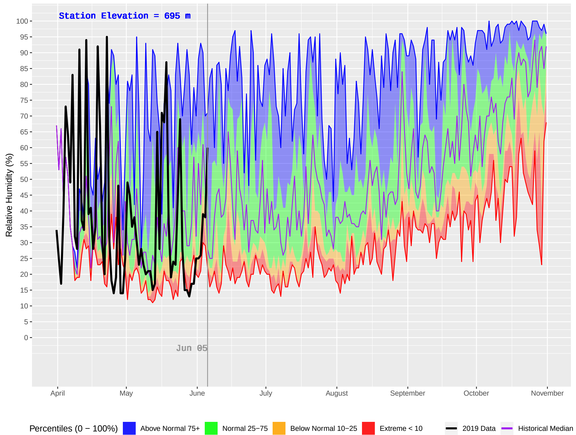
BLUE RIVER 2 (1108) : Historical (2011–2018) and Current (2019) Daily Relative Humidity
