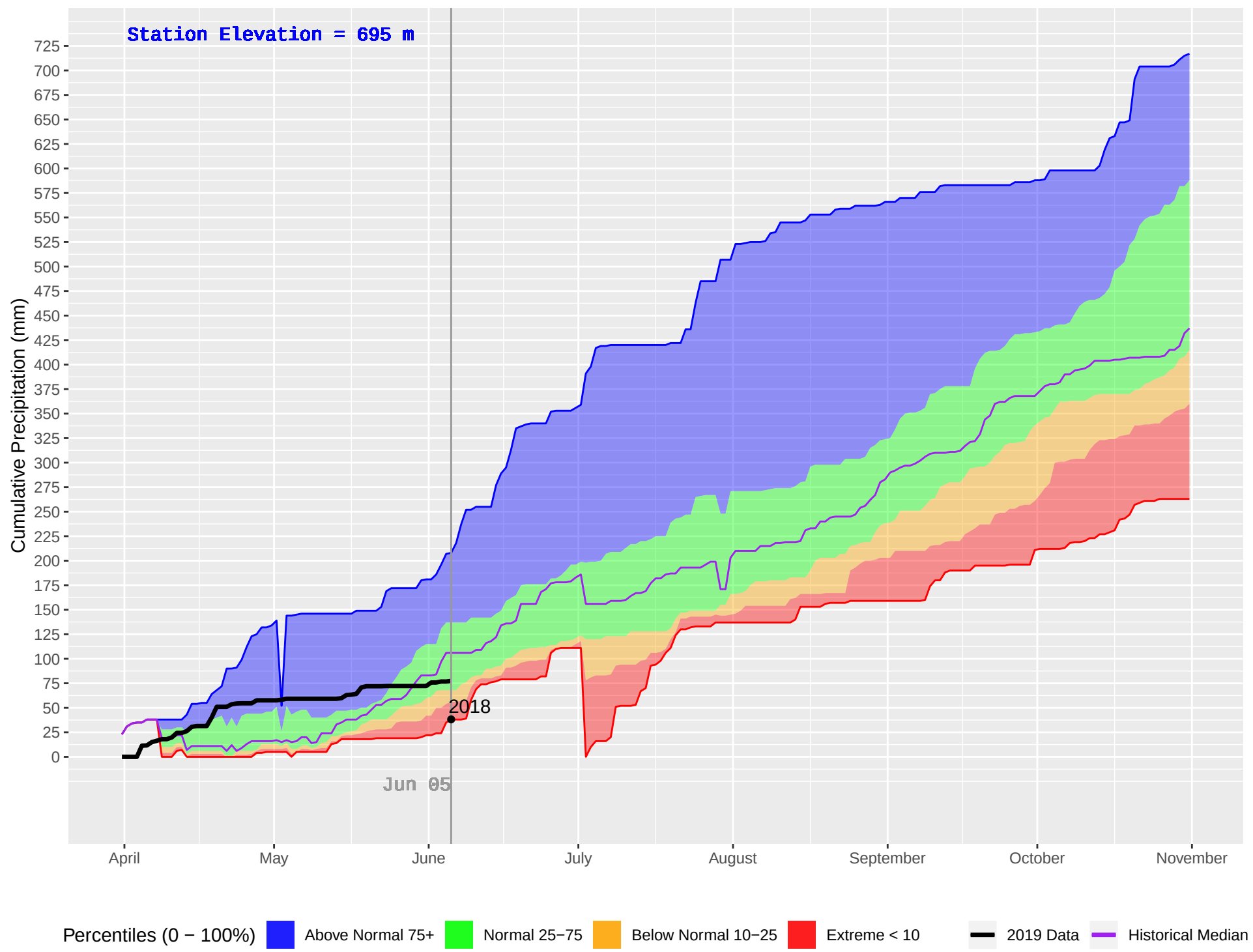
BLUE RIVER 2 (1108) : Historical (2011–2018), Current (2019) Daily Cumulative Precipitation
