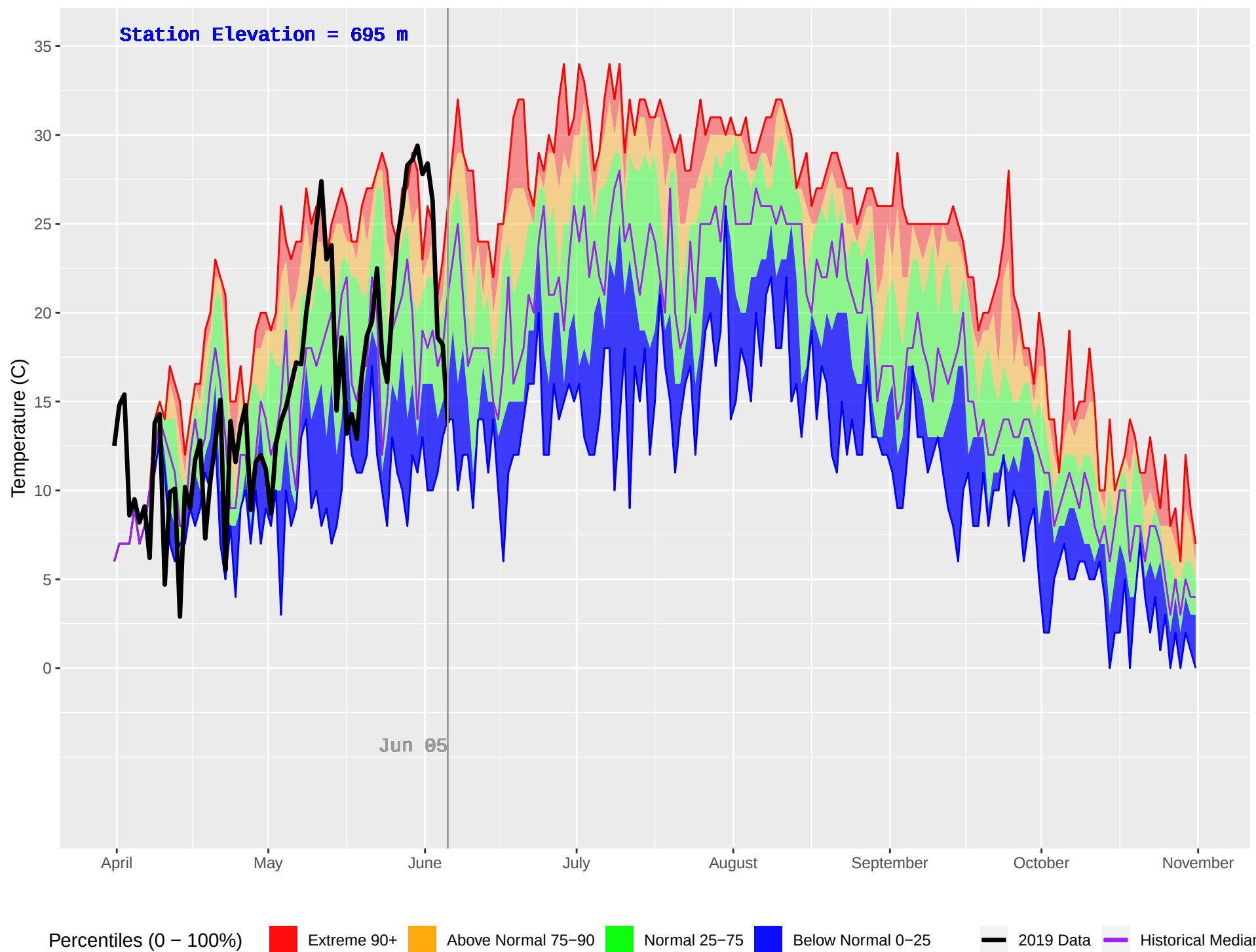
BLUE RIVER 2 (1108) : Historical (2011–2018) and Current (2019) Daily Temperature
