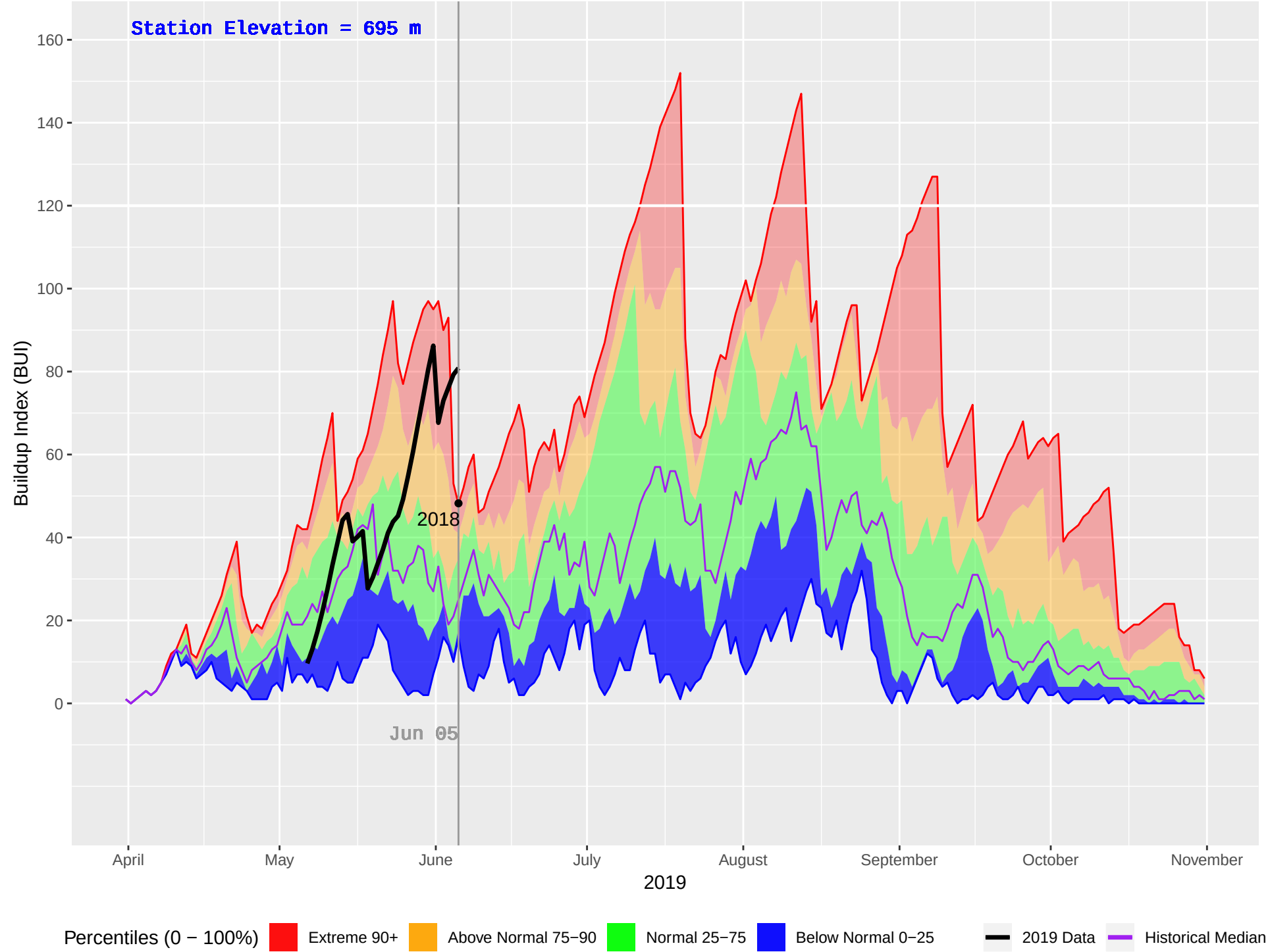
BLUE RIVER 2 (1108) : Historical (2011–2018), Current (2019) Daily Buildup Index (BUI)
