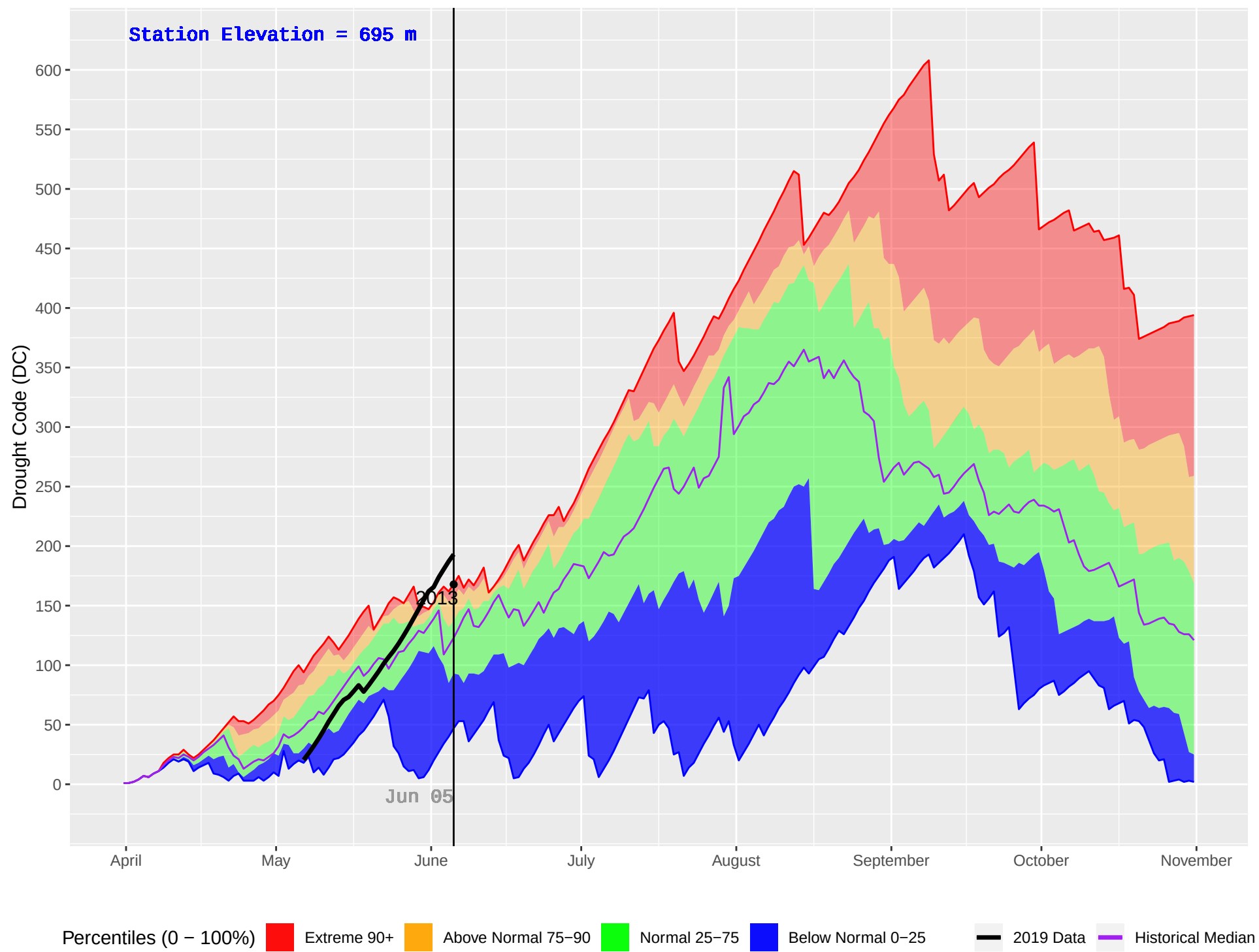
BLUE RIVER 2 (1108) : Historical (2011–2018) and Current (2019) Daily Drought Code (DC)
